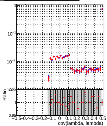
(PacketCandidate::bestTrack() - reco::Track)(reco::Track in cov(lambda, lambda) with over and underflow, and sign flip)
