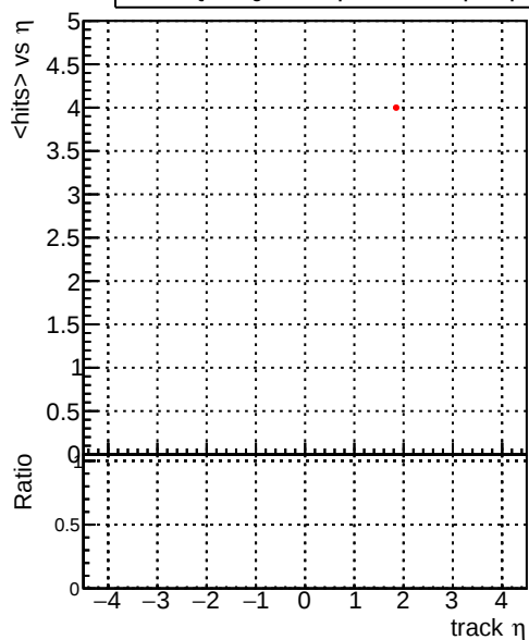
mean hits — DQM_correctCheck_mu_pt1to1000_eta1p5to2p0 — DQM_original_mu_pt1to1000_eta1p5to2p0
