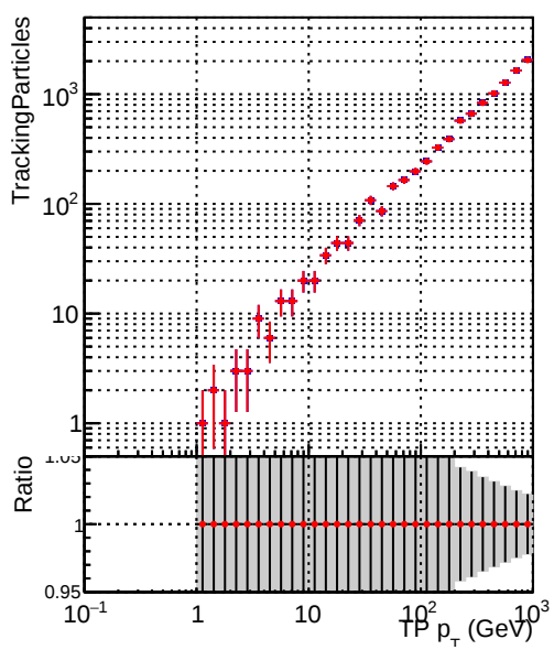
Legend: DQM_correctCheck_mu_pt1to1000_eta1p5to2p0 (blue line), DQM_original_mu_pt1to1000_eta1p5to2p0 (red line)
