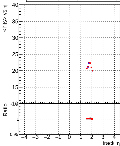
— DQM_correctCheck_mu_pt1to1000_eta1p5to2p0 — DQM_original_mu_pt1to1000_eta1p5to2p0
