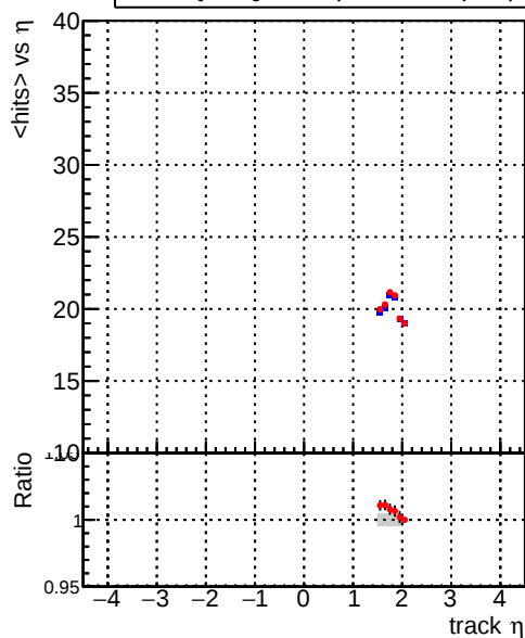
mean hits vs \eta — DQM_correctCheck_mu_pt1to1000_eta1p5to2p0 — DQM_original_mu_pt1to1000_eta1p5to2p0
