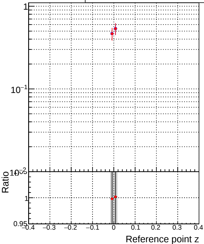
PackedCandidate::bestTrack()
