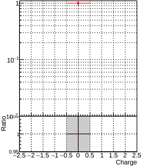
PackedCandidate DQM_correctCheck_mu_pt1to1000_eta1p0to1p5 DQM_original_mu_pt1to1000_eta1p0to1p5
