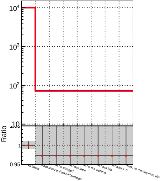
PackedCandidate DQM_correctCheck_mu_pt1to1000_eta1p0to1p5 DQM_original_mu_pt1to1000_eta1p0to1p5
