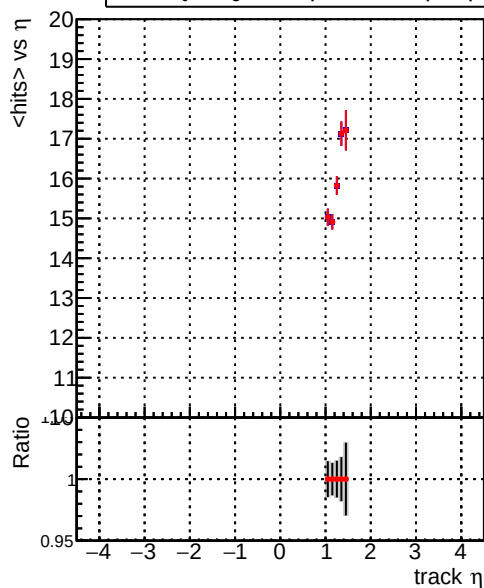
mean hit — DQM_correctCheck_mu_pt1to1000_eta1p0to1p5 — DQM_original_mu_pt1to1000_eta1p0to1p5
