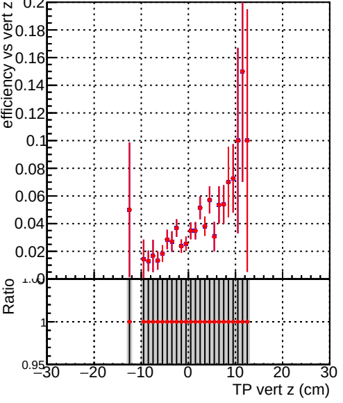
Efficiency vs TP vert z (cm) DQM_correctCheck_mu_pt1to1000_eta1p0to1p5 DQM_original_mu_pt1to1000_eta1p0to1p5
