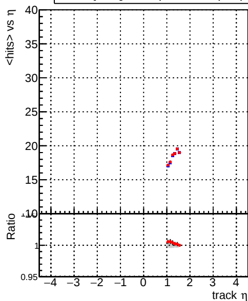
— DQM_correctCheck_mu_pt1to1000_eta1p0to1p5 — DQM_original_mu_pt1to1000_eta1p0to1p5
