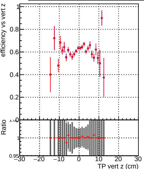
Efficiency vs TP vert z (cm) Legend: DQM_correctCheck_mu_pt0p1to1_eta2p0to2p5 DQM_original_mu_pt0p1to1_eta2p0to2p5
