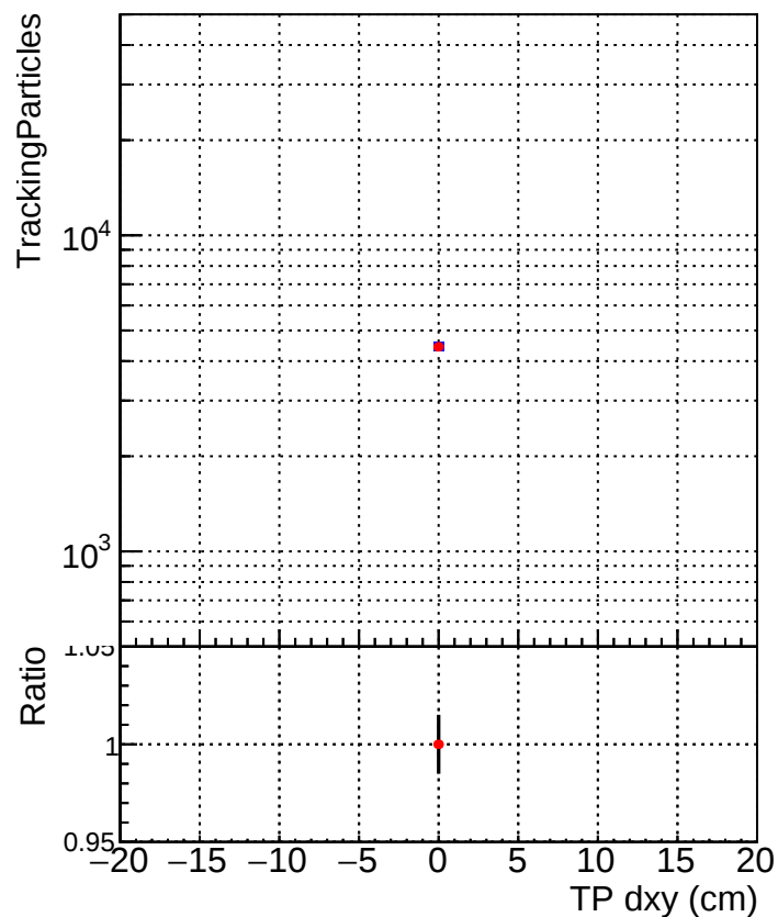
■ DQM_correctCheck_mu_pt0p1to1_eta2p0to2p5 ● DQM_original_mu_pt0p1to1_eta2p0to2p5
