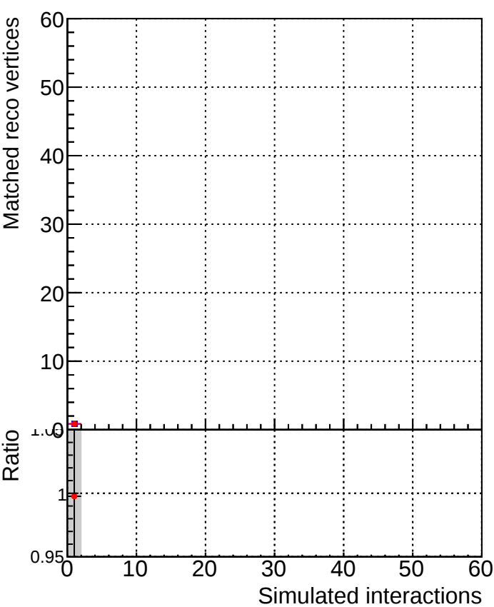
DQM_correctCheck_mu_pt0p1to1_eta2p0to2p5 DQM_original_mu_pt0p1to1_eta2p0to2p5
