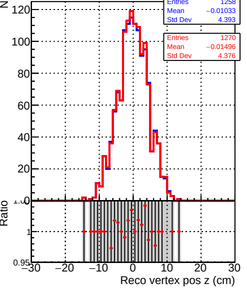
Recons DQM_correctCheck_mu_pt0p1to1_eta2p0to2p5 DQM_original_mu_pt0p1to1_eta2p0to2p5
