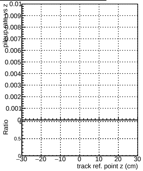
Legend: —•— DQM_correctCheck_mu_pt0p1to1_eta2p0to2p5 —•— DQM_original_mu_pt0p1to1_eta2p0to2p5
