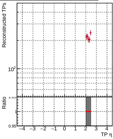
Legend: DQM_correctCheck_mu_pt0p1to1_eta2p0to2p5 (blue line with dots), DQM_original_mu_pt0p1to1_eta2p0to2p5 (red line with dots)
