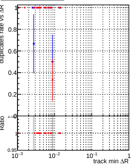
DQM_correctCheck_mu_pt0p1to1_eta2p0to2p5 DQM_original_mu_pt0p1to1_eta2p0to2p5
