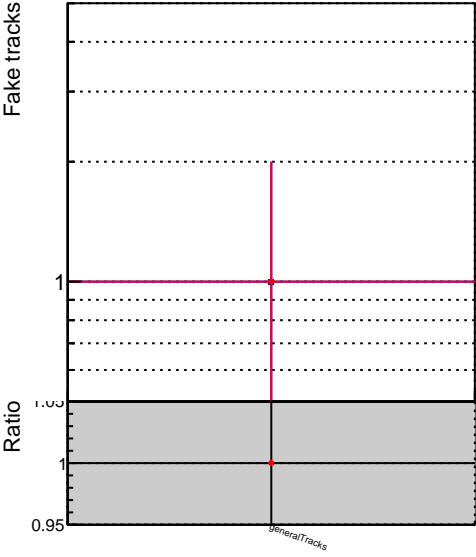
Number of tracks vs collection Legend: DQM_correctCheck_mu_pt0p1to1_eta2p0to2p5 (blue line), DQM_original_mu_pt0p1to1_eta2p0to2p5 (red line)
