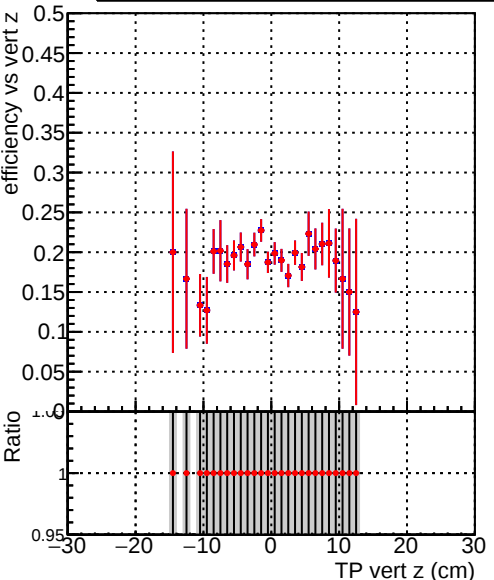
Efficiency vs TP vert z (cm) Legend: DQM_correctCheck_mu_pt0p1to1_eta1p5to2p0 DQM_original_mu_pt0p1to1_eta1p5to2p0
