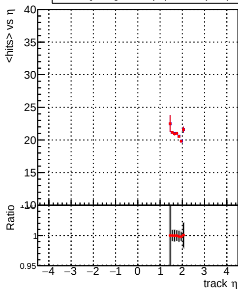
— DQM_correctCheck_mu_pt0p1to1_eta1p5to2p0 — DQM_original_mu_pt0p1to1_eta1p5to2p0
