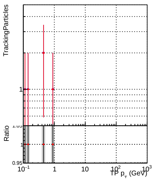
Legend: — DQM_correctCheck3_mu_pt1to1000_eta2p5to4p0 — DQM_original_mu_pt1to1000_eta2p5to4p0
