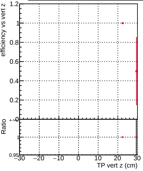
Efficiency vs TP vert z (cm) Legend: DQM_correctCheck3_mu_pt1to1000_eta2p5to4p0 DQM_original_mu_pt1to1000_eta2p5to4p0
