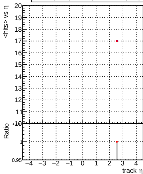
mean hits — DQM_correctCheck3_mu_pt1to1000_eta2p5to4p0 — DQM_original_mu_pt1to1000_eta2p5to4p0
