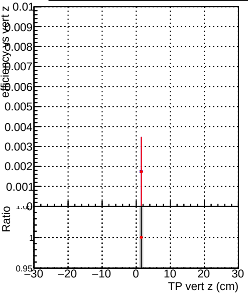
Efficiency vs vert z Legend: DQM_correctCheck3_mu_pt1to1000_eta2p5to4p0 (blue line with dots) DQM_original_mu_pt1to1000_eta2p5to4p0 (red line with dots)
