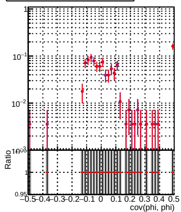
(PackedCandidate::bestTrack() - reco::Track)(reco::Track in cov(phi, phi) status and underflow and sign flip)
