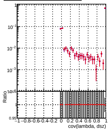
(PacketCandidate::bestTrack() - reco::Track)reco::Track in cov(lambda, dsz) not max
