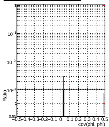
(PacketCandidate::bestTrack() - reco::Track)reco::Track in cov(phi, phi) not max
