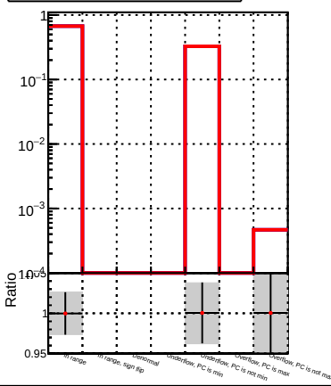
(PacketCandidate::bestTrack() - reco::Track)reco::Track in cov(qoverp, qoverp) status
