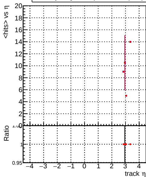
— DQM_correctCheck3_mu_pt1to1000_eta2p5to4p0 — DQM_original_mu_pt1to1000_eta2p5to4p0
