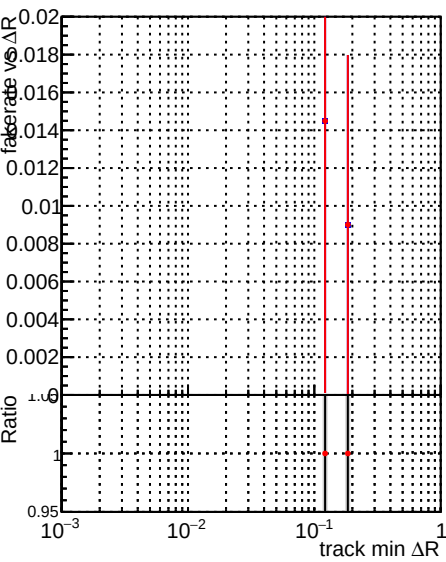
DQM_correctCheck3_mu_pt1to1000_eta2p5to4p0 DQM_original_mu_pt1to1000_eta2p5to4p0
