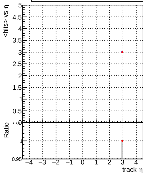
DQM_original_mu_pt1to1000_eta2p5to4p0
