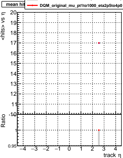
DQM_correctCheck3_mu_pt1to1000_eta2p5to4p0
