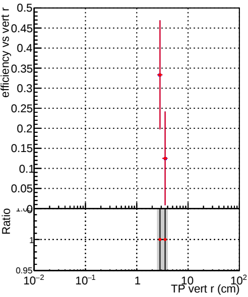
Efficiency vs vertpos Legend: DQM_correctCheck3_mu_pt1to1000_eta2p0to2p5 DQM_original_mu_pt1to1000_eta2p0to2p5
