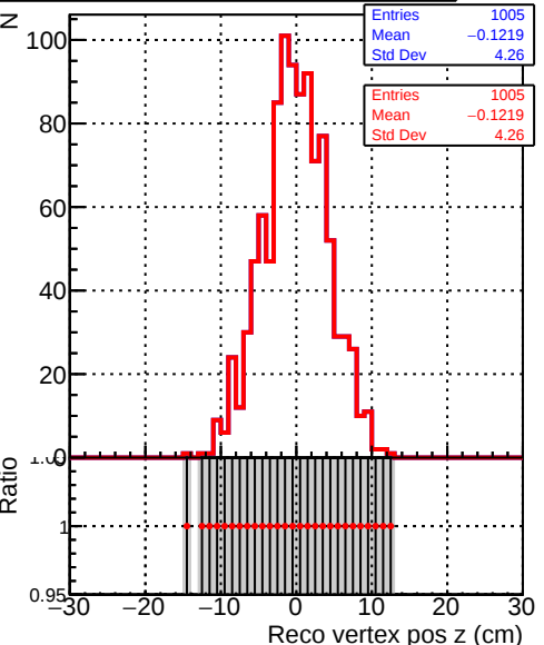
Recons DQM_correctCheck3_mu_pt1to1000_eta2p0to2p5 DQM_original_mu_pt1to1000_eta2p0to2p5
