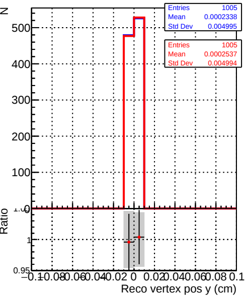
Recons DQM_correctCheck3_mu_pt1to1000_eta2p0to2p5 DQM_original_mu_pt1to1000_eta2p0to2p5
