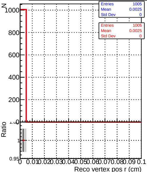
Recons DQM_correctCheck3_mu_pt1to1000_eta2p0to2p5 DQM_original_mu_pt1to1000_eta2p0to2p5
