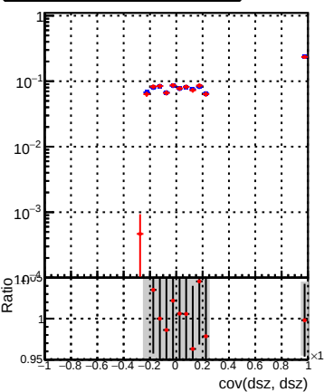
(PacketCandidate::bestTrack() - reco::Track)reco::Track in cov(dsz, dsz)
