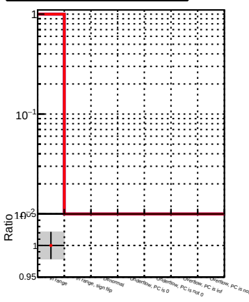
(PacketCandidate::bestTrack() - reco::Track)reco::Track in cov(dsz, dsz) status
