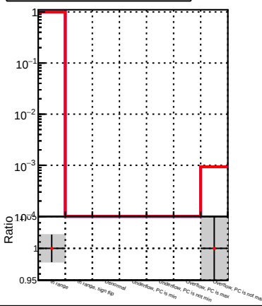
DQM_correctCheck3_mu_pt1to1000_eta2p0to2p5 DQM_original_mu_pt1to1000_eta2p0to2p5
