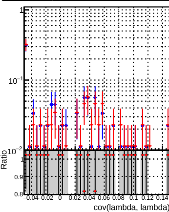
DQM_correctCheck3_mu_pt1to1000_eta2p0to2p5 DQM_original_mu_pt1to1000_eta2p0to2p5
