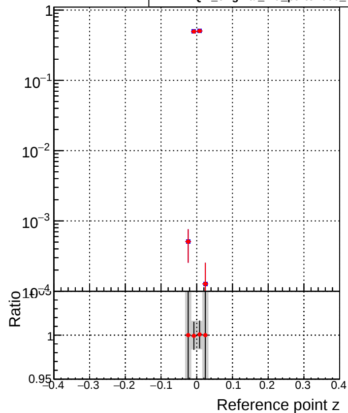
PackedCandidate::bestTrack
