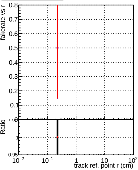
Fake rate vs v DQM_correctCheck3_mu_pt1to1000_eta2p0to2p5 DQM_original_mu_pt1to1000_eta2p0to2p5
