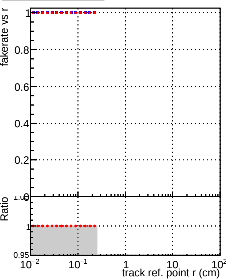
Fake rate vs verpos DQM_correctCheck3_mu_pt1to1000_eta2p0to2p5 DQM_original_mu_pt1to1000_eta2p0to2p5
