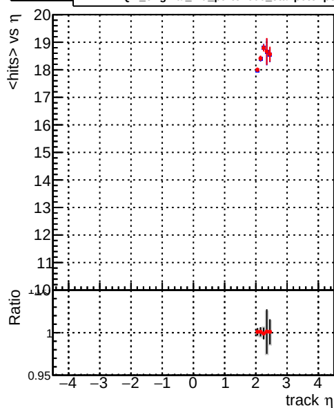
— DQM_correctCheck3_mu_pt1to1000_eta2p0to2p5 — DQM_original_mu_pt1to1000_eta2p0to2p5
