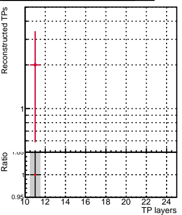
■ DQM_correctCheck3_mu_pt1to1000_eta2p0to2p5 ■ DQM_original_mu_pt1to1000_eta2p0to2p5
