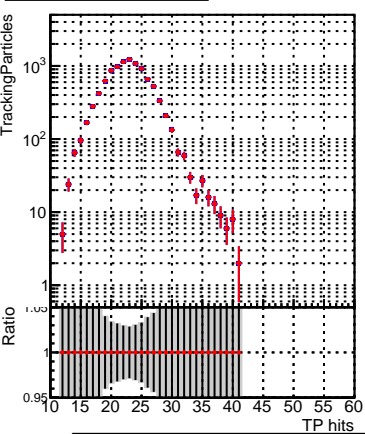
■ DQM_correctCheck3_mu_pt1to1000_eta2p0to2p5 ■ DQM_original_mu_pt1to1000_eta2p0to2p5
