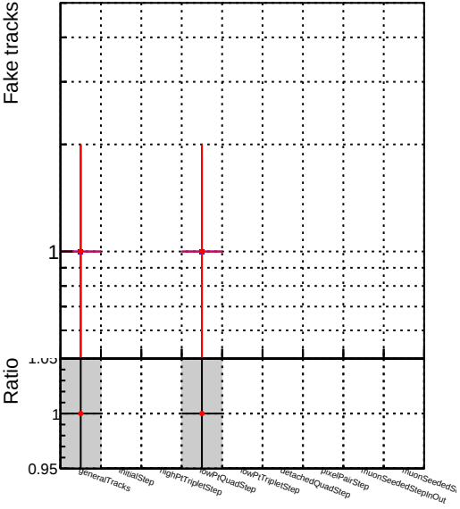
Legend: DQM_correctCheck3_mu_pt1to1000_eta1p5to2p0 (blue line with error bars), DQM_original_mu_pt1to1000_eta1p5to2p0 (red line with error bars)
