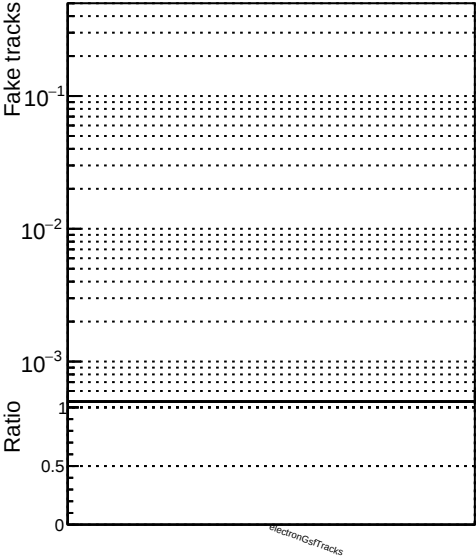
Number of fake tracks vs collection Legend: DQM_correctCheck3_mu_pt1to1000_eta1p5to2p0 DQM_original_mu_pt1to1000_eta1p5to2p0
