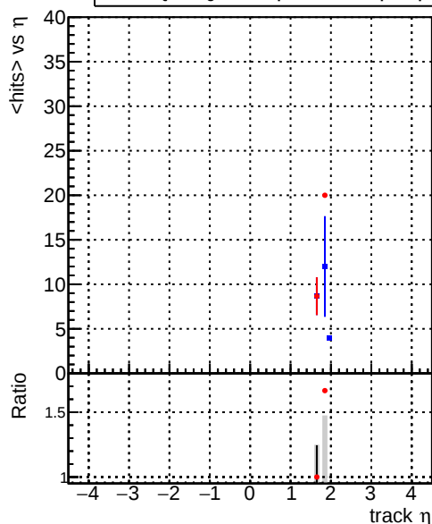
— DQM_correctCheck3_mu_pt1to1000_eta1p5to2p0 — DQM_original_mu_pt1to1000_eta1p5to2p0
