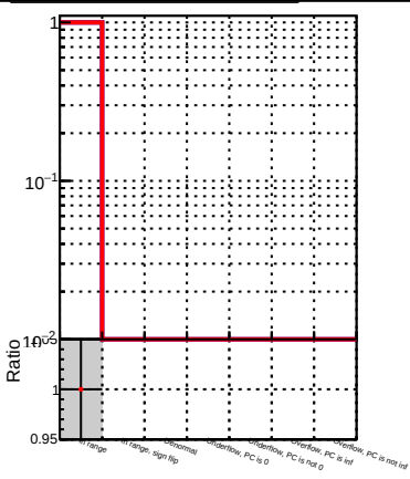
DQM_correctCheck3_mu_pt1to1000_eta1p0to1p5 DQM_original_mu_pt1to1000_eta1p0to1p5
