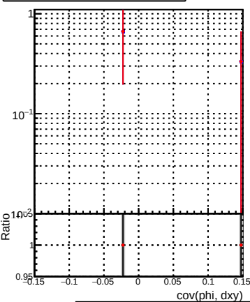
DQM_correctCheck3_mu_pt1to1000_eta1p0to1p5 DQM_original_mu_pt1to1000_eta1p0to1p5
