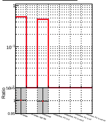
(PacketCandidate::bestTrack() - reco::Track)reco::Track in cov(dxy, dsz) status
