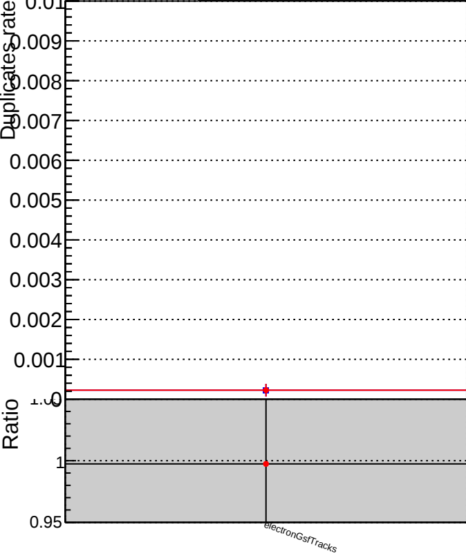
Duplicates rate vs collection Legend: DQM_correctCheck3_mu_pt1to1000_eta1p0to1p5 DQM_original_mu_pt1to1000_eta1p0to1p5
