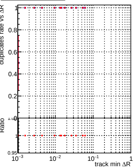
Legend: DQM_correctCheck3_mu_pt1to1000_eta1p0to1p5 DQM_original_mu_pt1to1000_eta1p0to1p5
