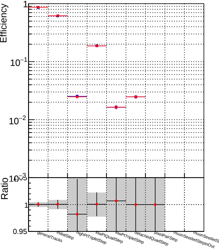
DQM_correctCheck3_mu_pt0p1to1_eta2p0to2p5 DQM_original_mu_pt0p1to1_eta2p0to2p5
