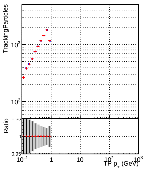
Legend: DQM_correctCheck3_mu_pt0p1to1_eta2p0to2p5 (blue line with dots), DQM_original_mu_pt0p1to1_eta2p0to2p5 (red line with dots)
