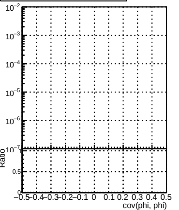
(PacketCandidate::bestTrack() - reco::Track)reco::Track in cov(phi, phi) with over and underflow, and sign flip
