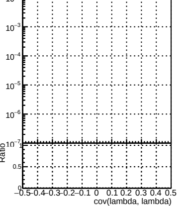
(PacketCandidate::bestTrack() - reco::Track)reco::Track in cov(lambda, lambda) with over and underflow, and sign flip
