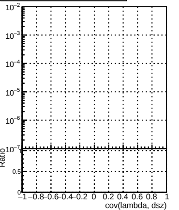
(PacketCandidate::bestTrack() - reco::Track)reco::Track in cov(lambda, dsz) with over and underflow, and sign flip
