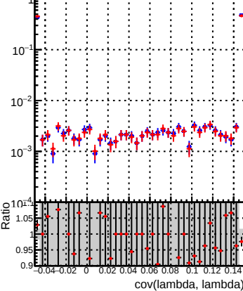
(PacketCandidate::bestTrack() - reco::Track)reco::Track in cov(lambda, lambda)
