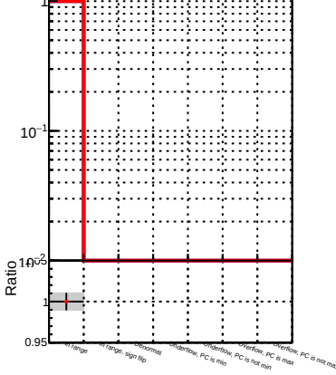
(PacketCandidate::bestTrack() - reco::Track)reco::Track in cov(lambda, lambda) status
