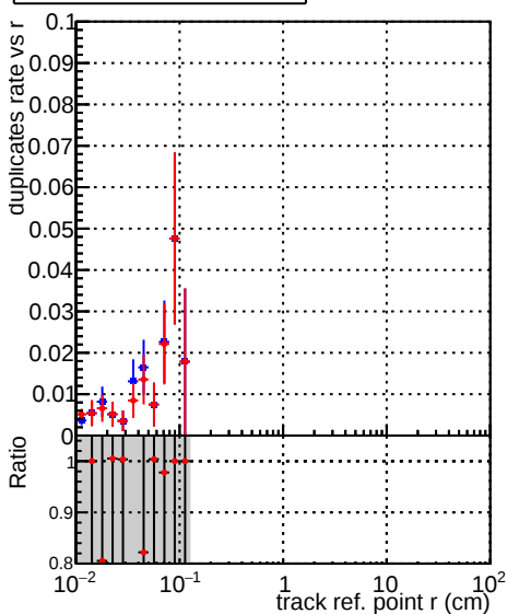
—•— DQM_correctCheck3_mu_pt0p1to1_eta2p0to2p5 —•— DQM_original_mu_pt0p1to1_eta2p0to2p5
