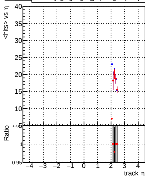
— DQM_correctCheck3_mu_pt0p1to1_eta2p0to2p5 — DQM_original_mu_pt0p1to1_eta2p0to2p5
